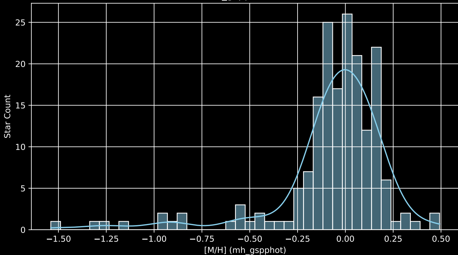
APOGEE DR17 Field: [045-06 [M/H] (mh_gspphot) (n= 182)
