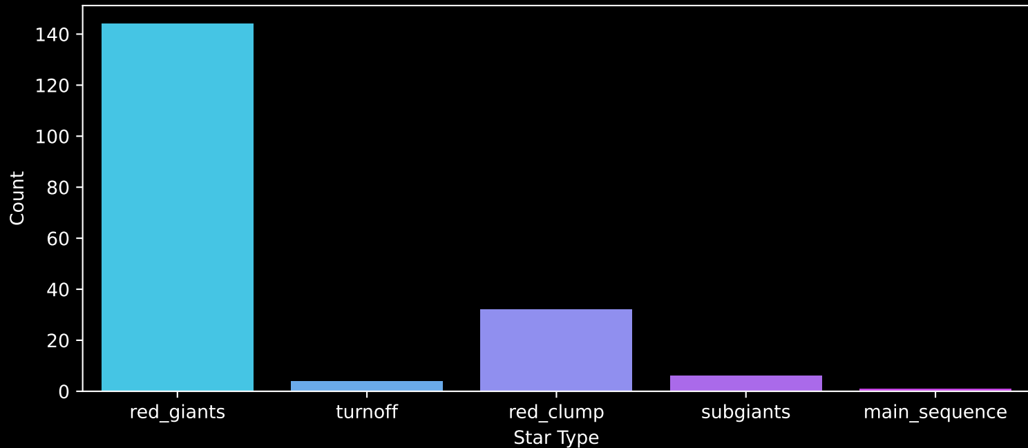
APOGEE DR17 Field: [045-06] Count plot of Star Type
