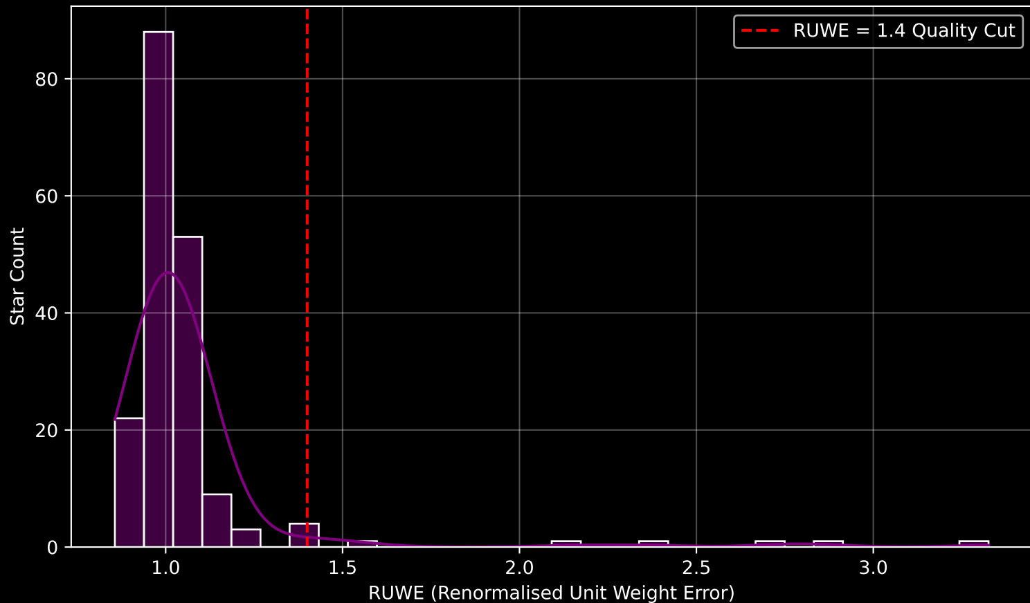
GAPOGEE DR17 Field [045-06] RUWE Distribution (n= 185)
