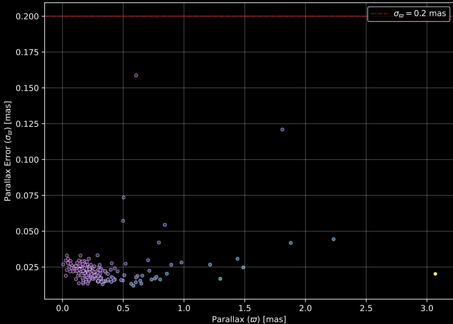
APOGEE DR17 Field: [045-06] Parallax Quality (n= 187)
