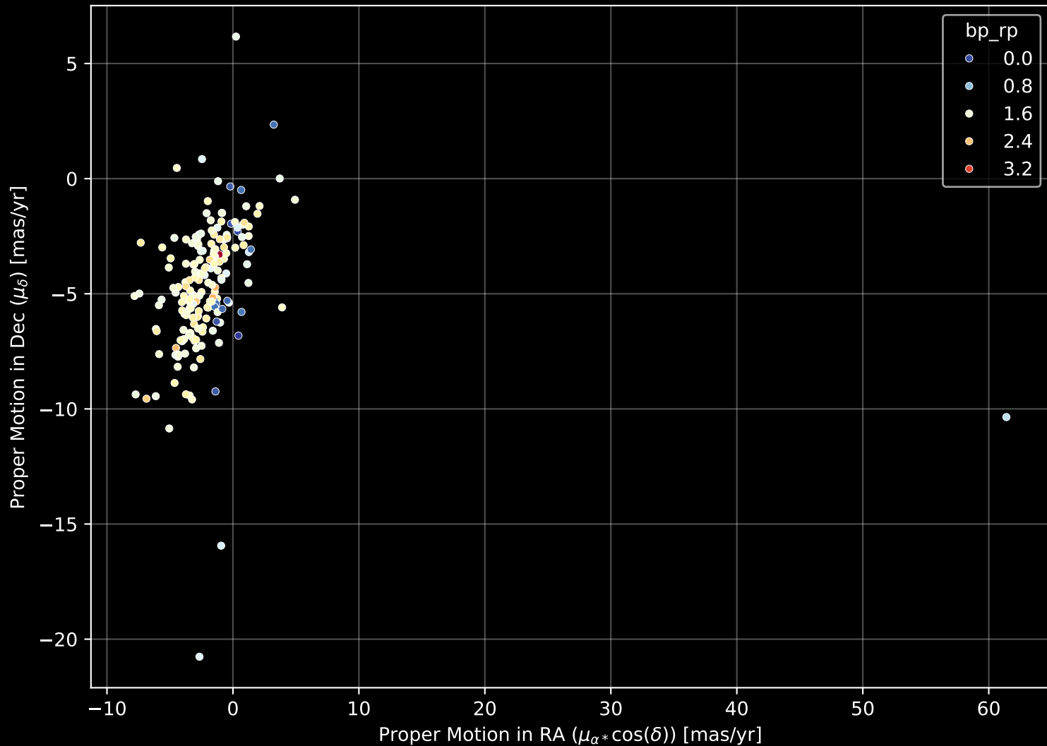
APOGEE DR17 Field: [045-06] Proper Motion Diagram (n= 187)
