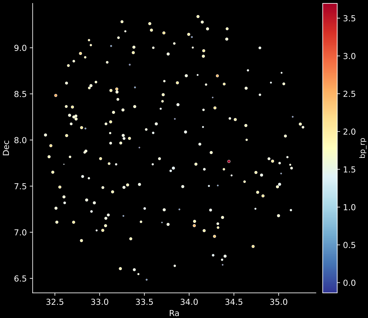
APOGEE DR17 Field: [045-06] Stars: 187
