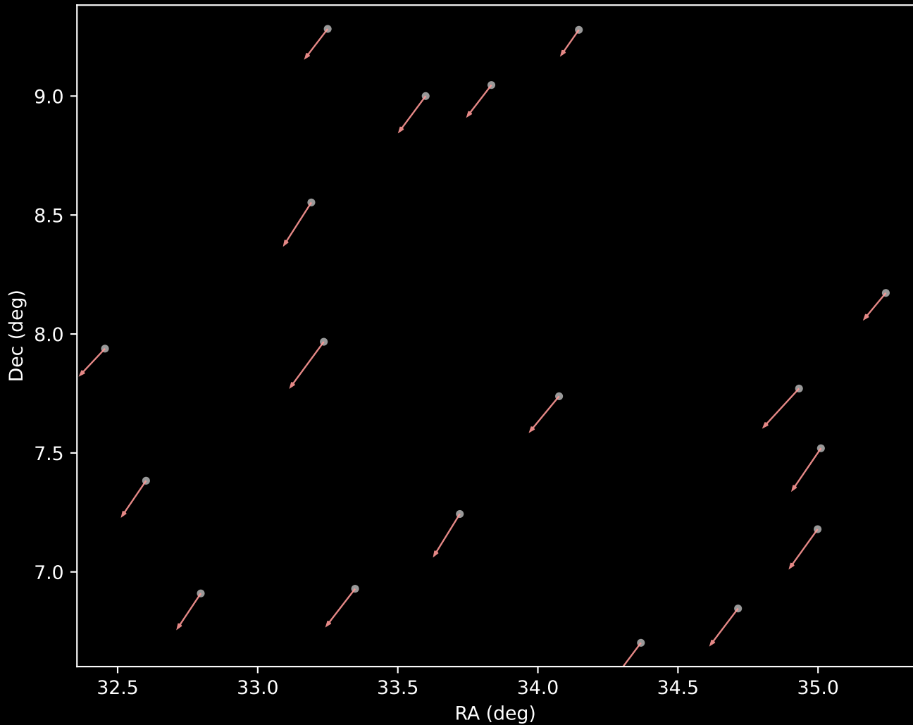
APOGEE DR17 Cluster 7 Proper Motion Vectors (n=18)
